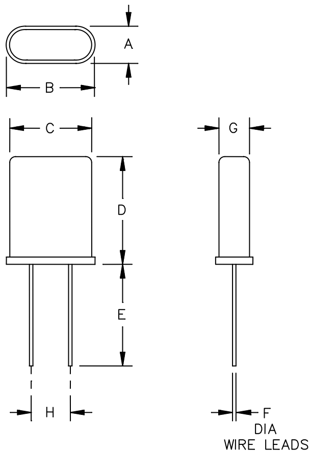
FIGURE 1. Crystal unit - CR60/U.
