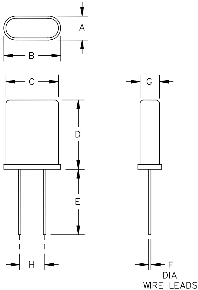
FIGURE 1. Crystal unit - CR97/U.
